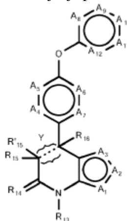
(Formula I)
