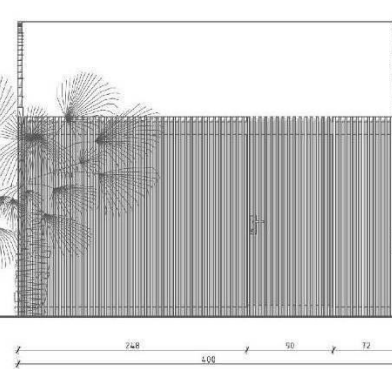
pogled 3, R 1:50
