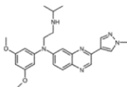
(I), (JNJ-42756493)
