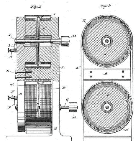
(No Model.) N. TESLA. DYNAMO ELECTRIC MACHINE. No. 406,968. Patented July 16, 1889.
