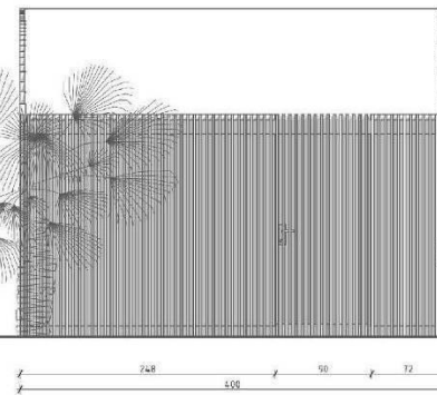
pogled 3, R 1:50
