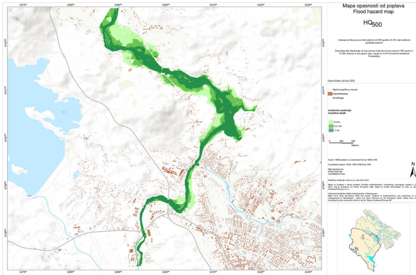
Figure 0-2. Inundation Depth (HQ500) for APSFR20_ARB_Zeta01 (Northern Region)
