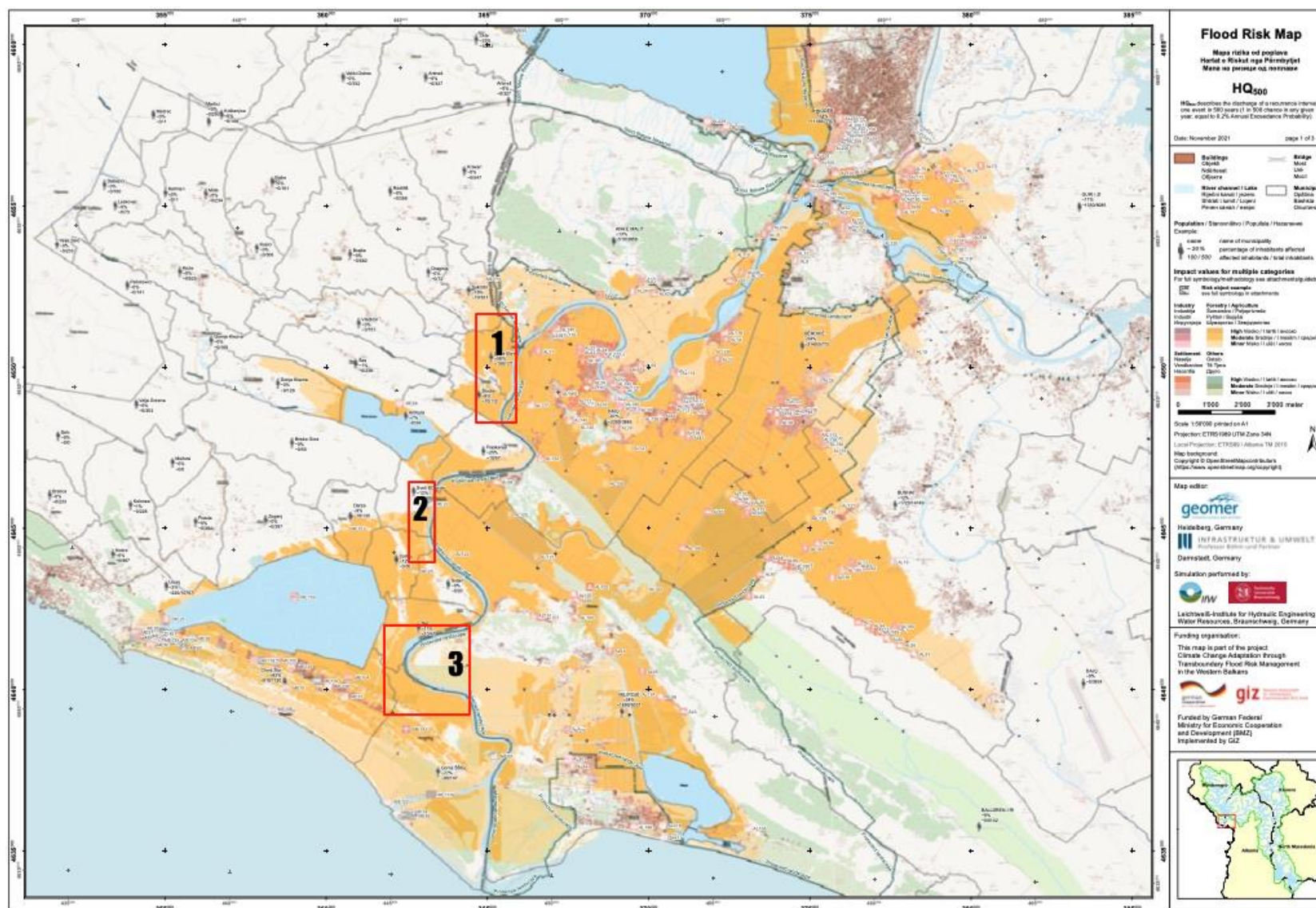
Figure 8.4. Identified areas of potential flooding in APSFR25_ARB_Bojana01
