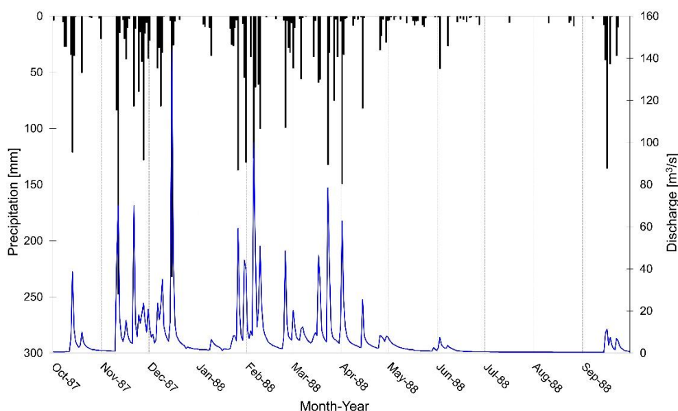
Figure B. Hydrograph of Rijeka Crnojevića spring discharge (hydrometric station "Brodka Njiva") with precipitation bar graph (climatological station "Cetinje") 69
