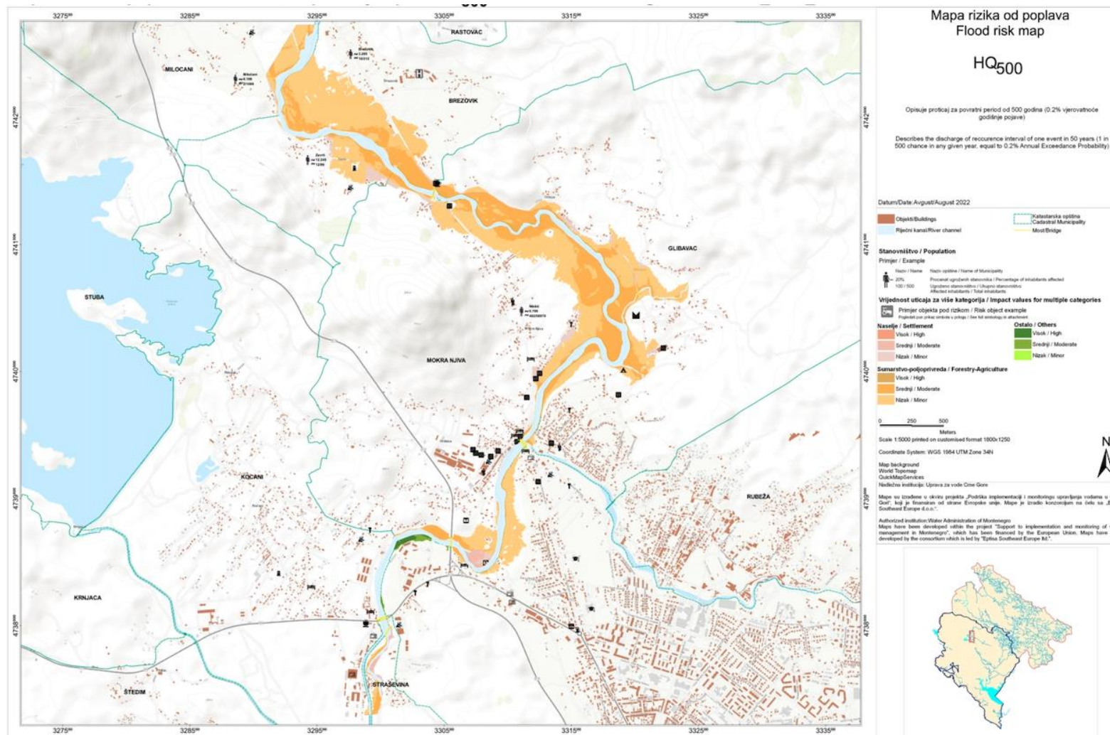
Figure 6.4. Flood Extent for APSFR20_ARB_Zeta01 (Southern Region)
