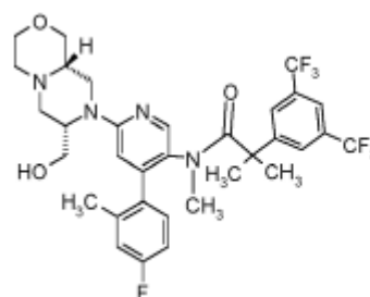
(Compound A)
