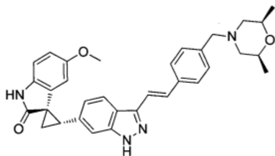
Compound (I)
