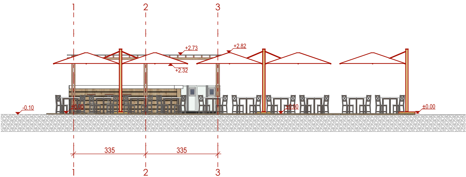
A Elevation 1:100
